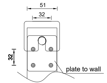
Wall hang illustration
