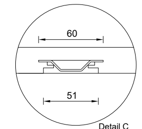
Detail C Built in wall bracket plate
