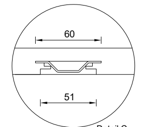
Detail C Built in wall bracket plate
