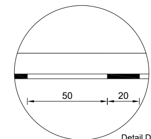
Detail D Drainage Line
