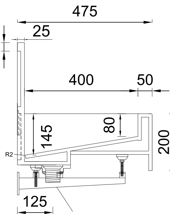
cantilever wall brackets
