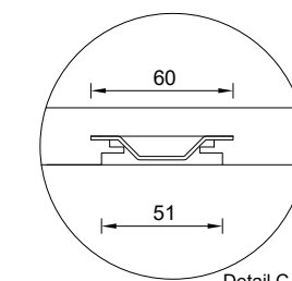
Detail C Built in wall bracket plate
