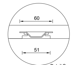
Detail C Built in wall bracket plate
