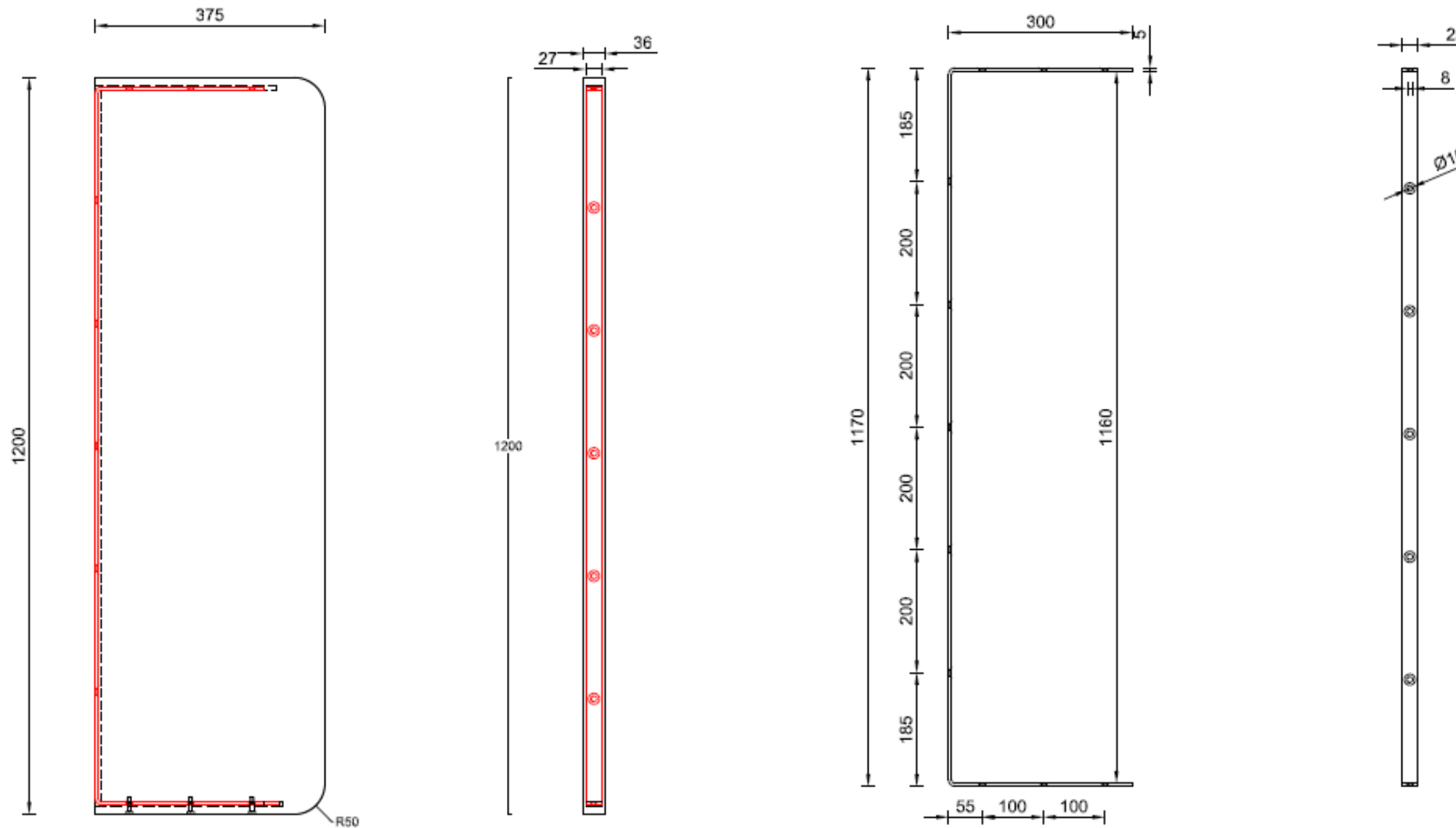
Corian® Urinal Divider Panel with concealed U plate
